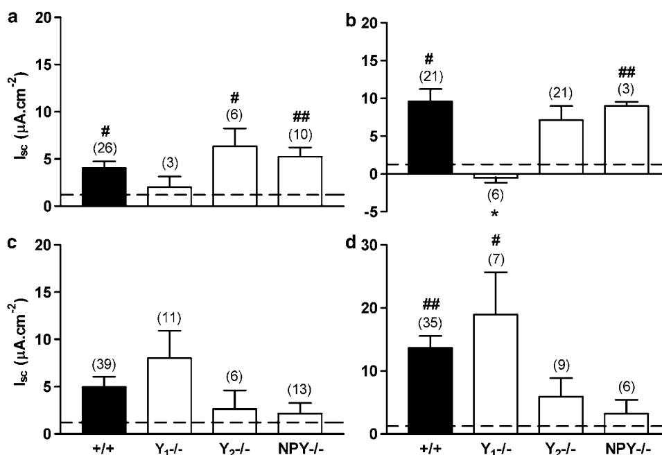
Figure 8 Blockade of endogenous Y_1 -inhibitory tone (by BIBO3304, 300 nM) in (a): untreated controls, or (b): following VIP (30 nM) pretreatment of different genotype mouse colon mucosae. Inhibition of Y_2 -inhibitory tone (with BIIE0246, 1 \mu M ) in naive (c) or VIP-pretreated (d) wild-type ( +/+ ), Y_1^{-/-} , Y_2^{-/-} or NPY ^{-/-} colon mucosae. The dashed line in all histograms represents the vehicle control (DMSO, 0.01%). Data are the mean \pm 1 s.e.m. with n numbers shown in parenthesis. A one-way ANOVA using Dunnett's post-test was used to compare +/+ responses with those in -/- tissues, and *P \leq 0.05 was considered significant. A Student's unpaired t -test was used to compare BIBO3304 and BIIE0246 effects with vehicle controls and these significant differences are denoted by hatches (# P \leq 0.05 , ## P \leq 0.01 ).
