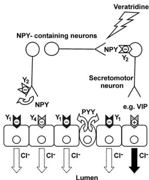
Figure 9 Schematic diagram depicting potential sites of action for neuronal NPY and endocrine PYY upon different targets in wild-type mouse descending colon mucosa. Veratridine nonselectively stimulates all intrinsic submucous neurons. Endocrine PYY may coactivate neuronal Y 2 receptors as well as epithelial Y 1 receptors, the latter predominating and resulting in a sustained inhibition of epithelial Cl - secretion. NPY released from submucosal secretomotor neurons can feedback to inhibit further NPY release (a Y 2 receptor-mediated effect) and also, when released from interneurons, can inhibit (again via Y 2 receptors) other NANC secretomotor neurons. The NANC neurotransmitter in this final secretomotor neuron cannot as yet be positively identified, but is most likely to be VIP. Stimulation of epithelial VIP receptors results in activation of epithelial Cl - secretion, while epithelial Y 1 (or Y 4 ) receptor activation will inhibit mucosal anion secretion.
