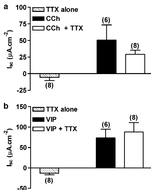
Figure 2 The effects of TTX pretreatment alone (100 nM, hatched bars) and upon subsequent CCh (10 \mu M , a) and VIP (30 nM, b) responses. Each bar is the mean \pm 1 s.e.m. with n numbers shown in parenthesis. Student's unpaired t -test was used to compare control and TTX-treated data groups for either agonist and no significant differences were observed.
