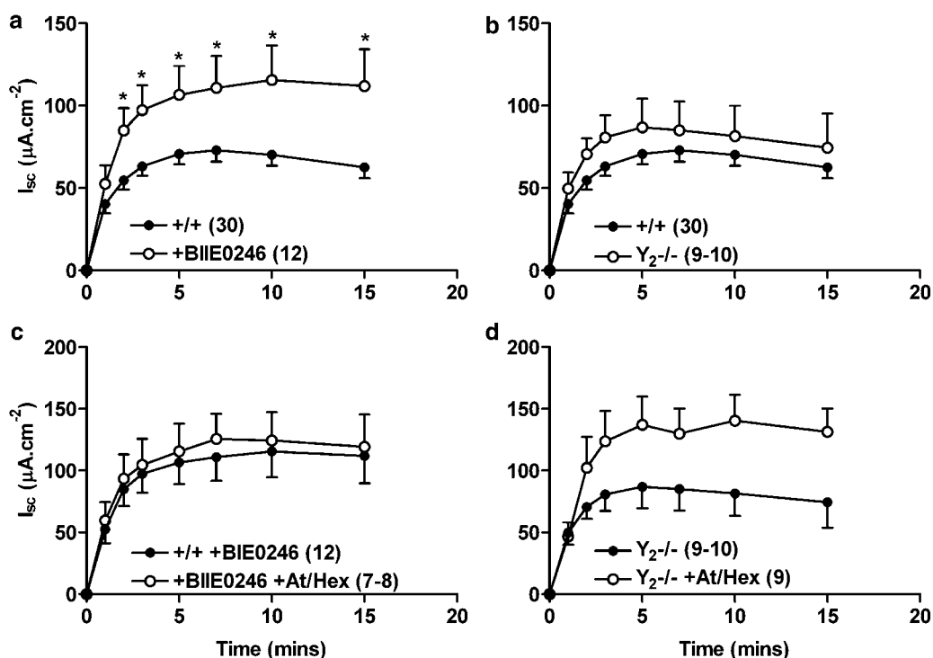
Figure 4 The effects of either Y_2 receptor antagonism (BIIE0246, 1 \mu M , a), or Y_2 receptor knockout ( Y_2^{-/-} , b) upon veratridine-induced I_{sc} responses compared with wild-type (+/+) controls. The effects of cholinergic blockade (atropine, At, 1 \mu M and hexamethonium, Hex, 10 \mu M ) upon BIIE0246-pretreated +/+ tissue (in c), or Y_2^{-/-} tissue (in d) are shown for comparison. Veratridine (30 \mu M ) was added at time 0 min. Each point is the mean \pm 1 s.e.m. and n numbers are given in parenthesis. A Student's unpaired t -test was used to compare individual time points and significant differences are shown; * P < 0.05 .
