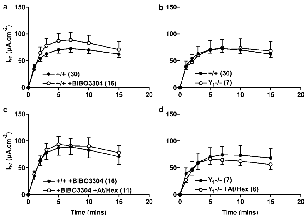
Figure 3 The effects of either Y_1 receptor antagonism (BIBO3304, 300 nM, in a) or Y_1 receptor knockout ( Y_1^{-/-} , in b) upon veratridine-induced (30 \mu M , added at time 0 min) I_{sc} responses. Cholinergic blockade with atropine (At, 1 \mu M ) and hexamethonium (Hex, 10 \mu M , c and d) did not significantly alter veratridine responses in either BIBO3304-pretreated tissue (c) or in Y_1^{-/-} tissue (d). Each pooled mucosal veratridine response was compared wild-type (+/+) responses. Data are the mean \pm 1 s.e.m. and n numbers are given in parenthesis.
