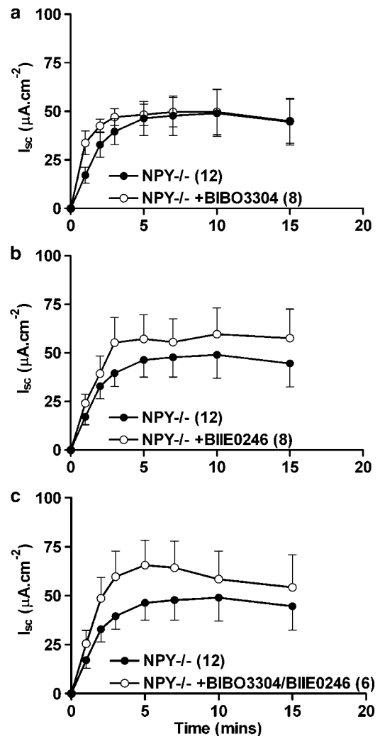
Figure 7 The effects of either single, Y_1 receptor antagonism (in a, BIBO3304, 300 nM) or in (b); Y_2 receptor blockade (BIIE0246, 1 \mu M) or in (c); combined Y_1 and Y_2 antagonism in NPY -/- colon throughout. Veratridine (30 \mu M) was added at time 0 min. Data are the mean \pm 1 s.e.m. with n numbers given in parenthesis. Student's unpaired t -test comparisons revealed there were no significant differences between any time points.
