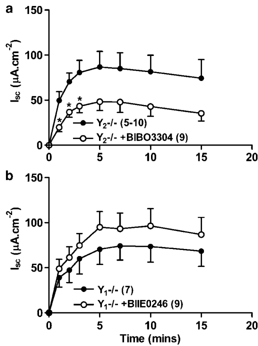
Figure 5 The effect of either Y_1 receptor antagonist pretreatment (BIBO3304, 300 nM) of Y_2 -/- colon (in a) or Y_2 antagonism (BIIE0246, 1 \mu M) of Y_1 -/- mucosa (in b). Veratridine (30 \mu M) was added at time 0 min and data are the mean \pm 1 s.e.m., with n numbers shown in parenthesis. A Student's unpaired t -test was used for comparison between individual pairs of time points in a; * P < 0.05.
