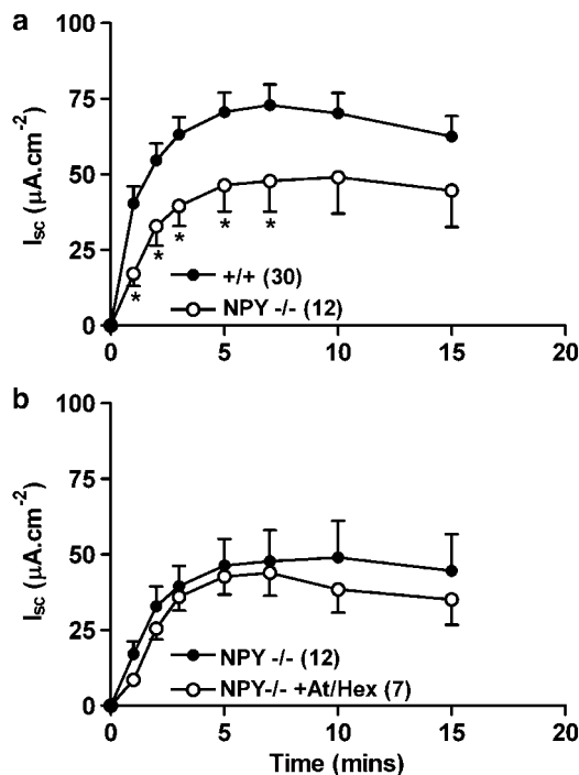
Figure 6 A comparison of NPY -/- and wild-type (+/+) colon mucosal veratridine responses in (a); and the effects of cholinergic blockade upon the same in NPY -/- colon in (b). Veratridine (30 \mu M) was added at time 0 min, and each data point is the mean \pm 1 s.e.m. with n numbers in parenthesis. A Student's unpaired t -test was used to compare individual pairs of time points and * P < 0.05.
