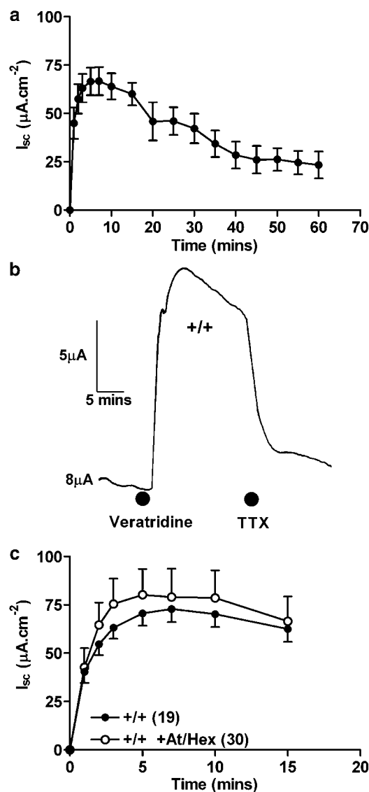
Figure 1 The pooled veratridine (30 \mu M ) I_{sc} responses over a period of 60 min (a) n=5-19 , and the sensitivity of a representative veratridine response to TTX (100 nM at 15 min, in b). In (c), a comparison of veratridine responses \pm cholinergic blockade with atropine (At, 1 \mu M ) and hexamethonium (Hex, 10 \mu M ) is shown. Numbers of observations are otherwise given in parenthesis and data (in a and c) is the mean \pm 1 s.e.m. A Student's unpaired t -test was used to compare veratridine responses \pm At/Hex and P>0.05 for all time points shown.
